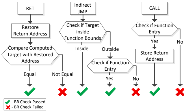
Fig. 2. Branch Regulation Checking Flow
