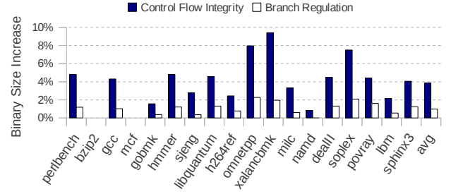
Fig. 10. Executable Size Increase
