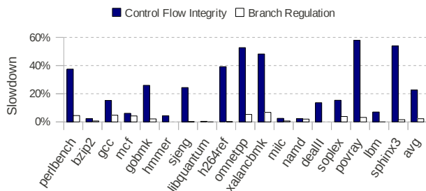
Fig. 12. Performance Overhead of Branch Regulation
