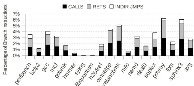
Fig. 13. Prevalence of Calls, Returns and Indirect Jumps
