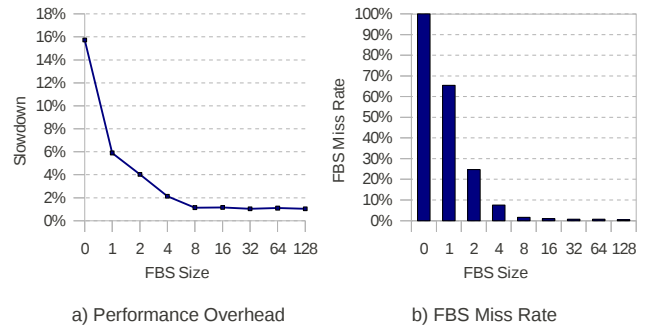
Fig. 11. Effect of FBS Size on Performance and FBS Miss Rate
