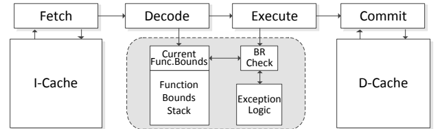
Fig. 6. Processor Pipeline with Branch Regulation Hardware
