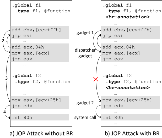
Fig. 1. Impact of BR on CRAs
