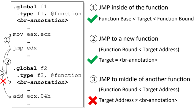
Fig. 5. Branch Regulation Checks
