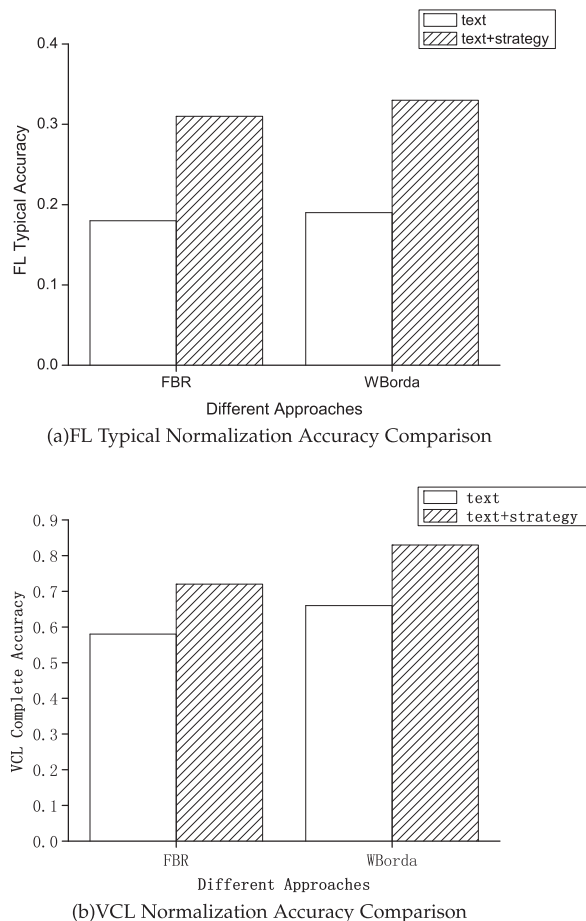
Fig. 5. Performance comparison of FBR and WBorda with and without strategy features on N-PVCD.
