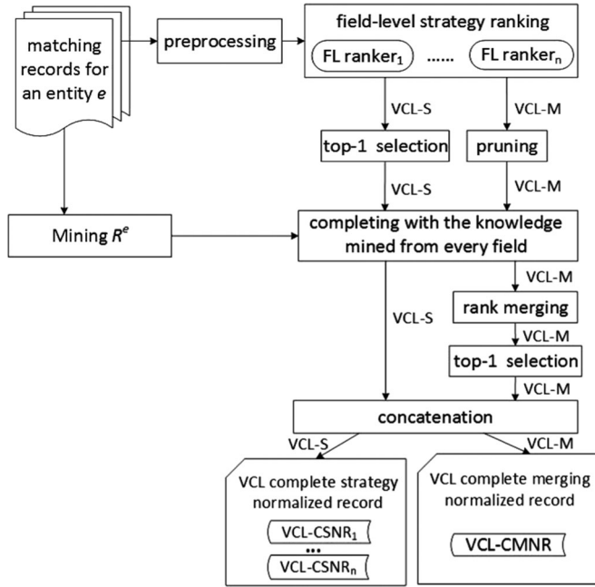
Fig. 2. The complete normalization framework.
