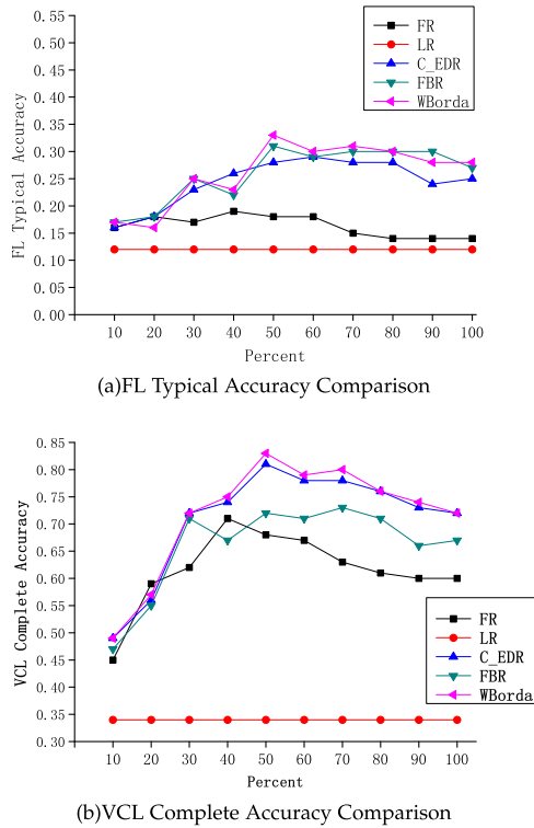
Fig. 3. Performance comparison by different approaches on a different percent of ranked results on N-PVCD.
