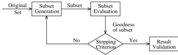
Fig. 1. Four key steps of feature selection.
