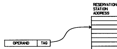
Figure 6 -- Tag Search Table for the DTS Algorithm.
