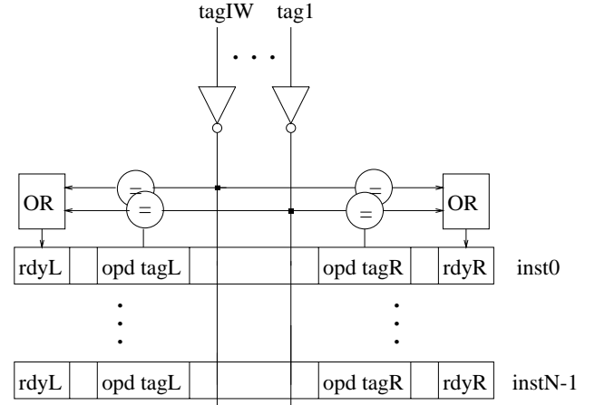
Figure 4: Wakeup logic.
