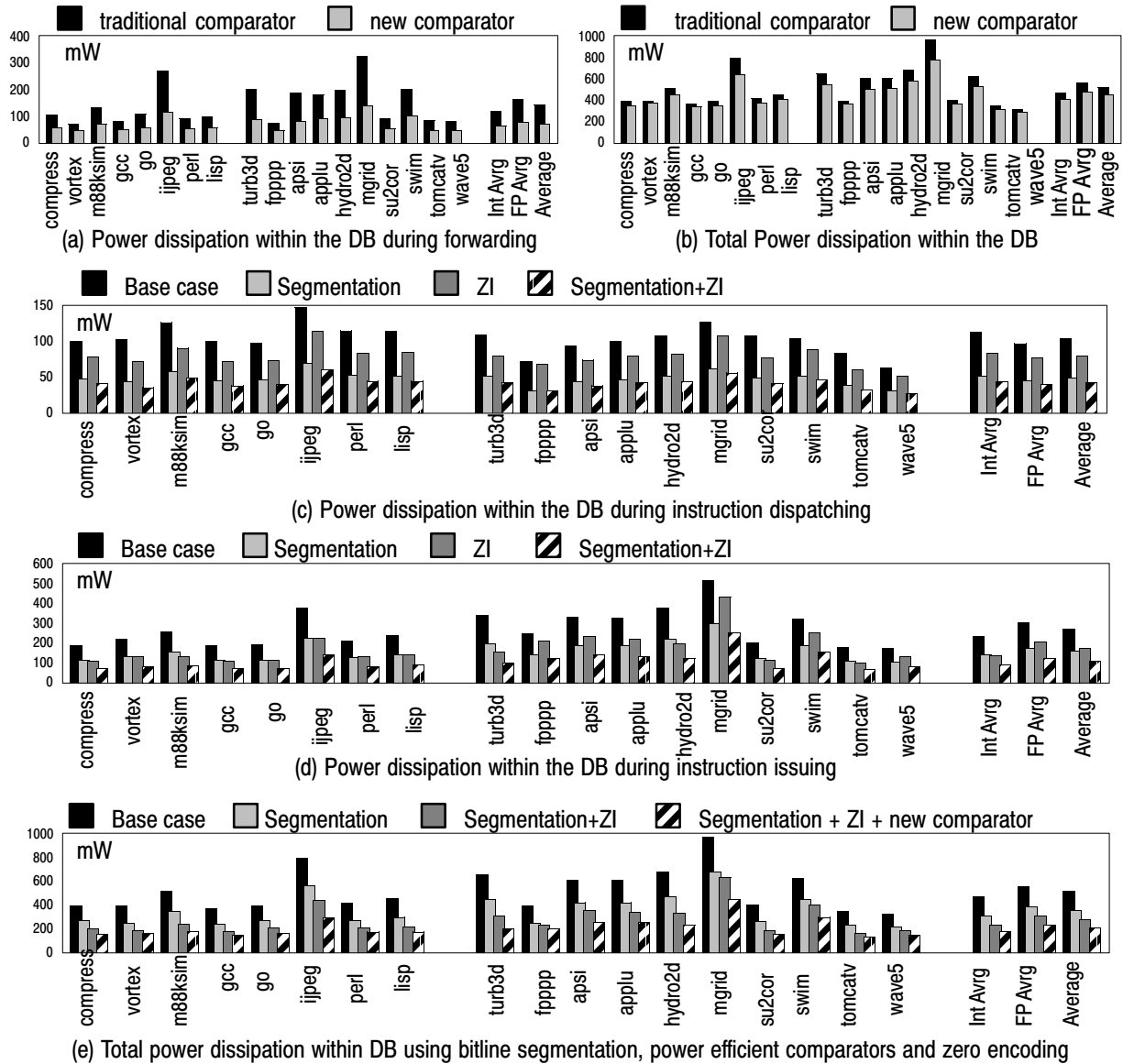
Figure 5. Power Savings Achieved in the Dispatch Buffer
