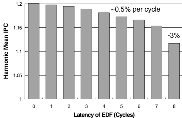
Figure 9. Latency tolerance of the EDF system of the slow window
