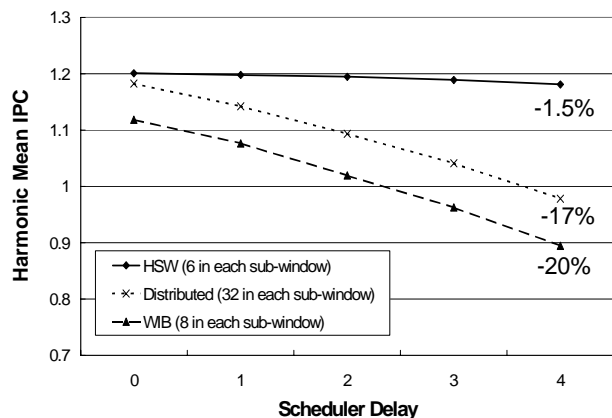
Figure 14. Scheduler latency tolerance comparison
