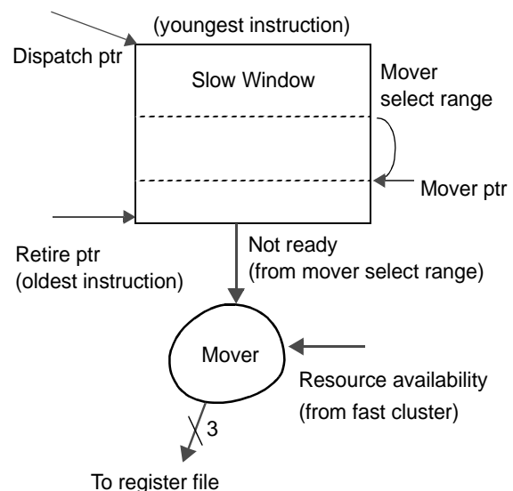
Figure 5. Mover implementation
