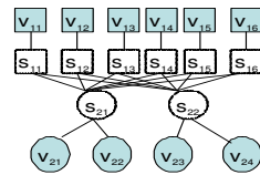
Figure 4: An RSN equivalent to k-means
