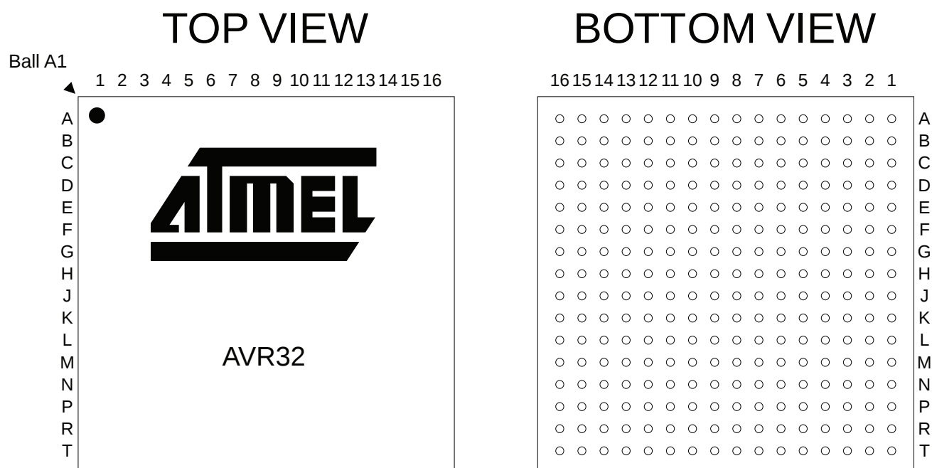
Figure 2-2. 256 CTBGA Pinout
