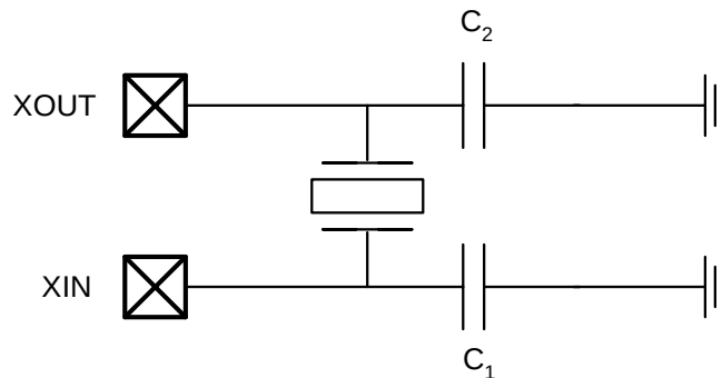
Figure 10-1. Oscillator connections
