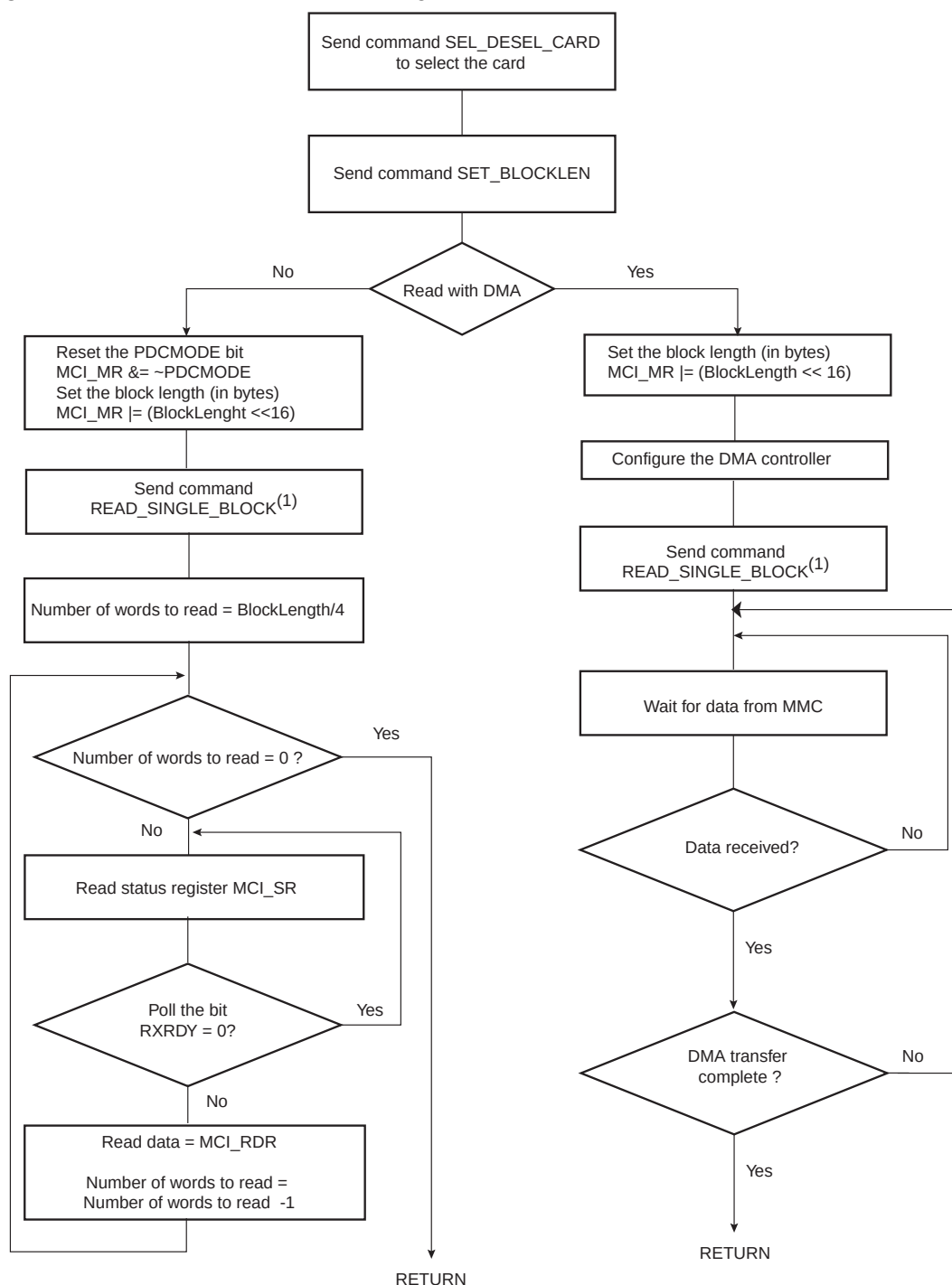
Figure 30-9. Read Functional Flow Diagram
