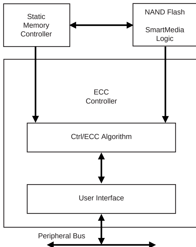
Figure 29-1. Block Diagram
