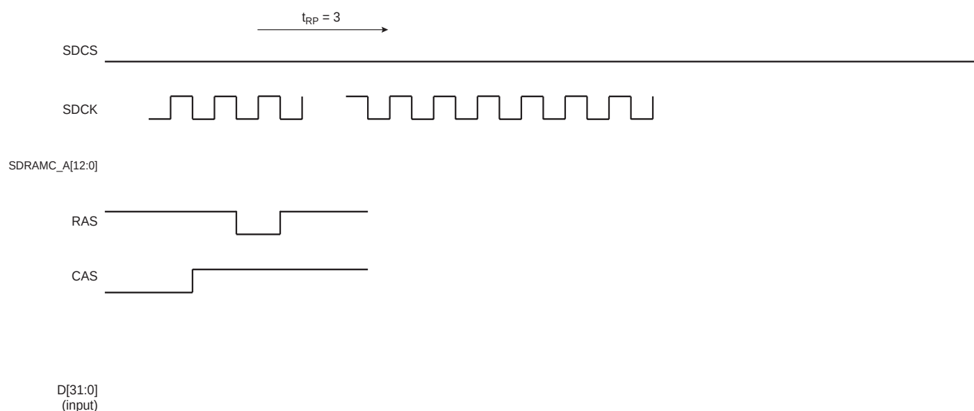
Figure 28-8. Refresh Cycle Followed by a Read Access
