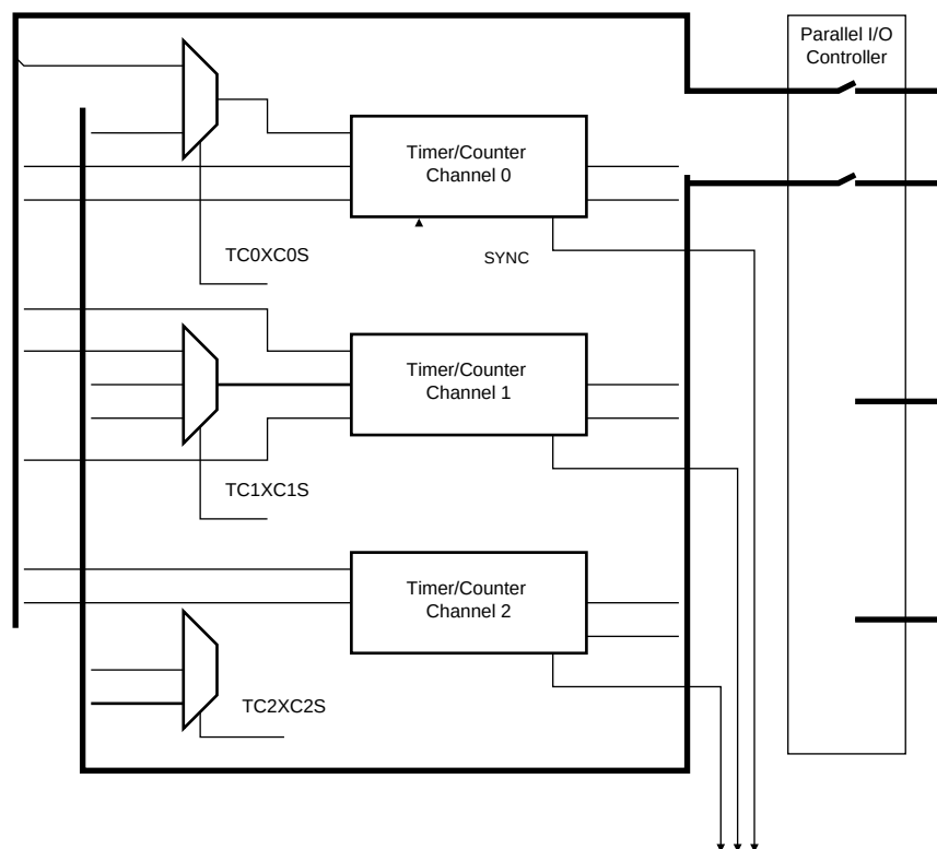
Figure 33-1. Timer Counter Block Diagram
