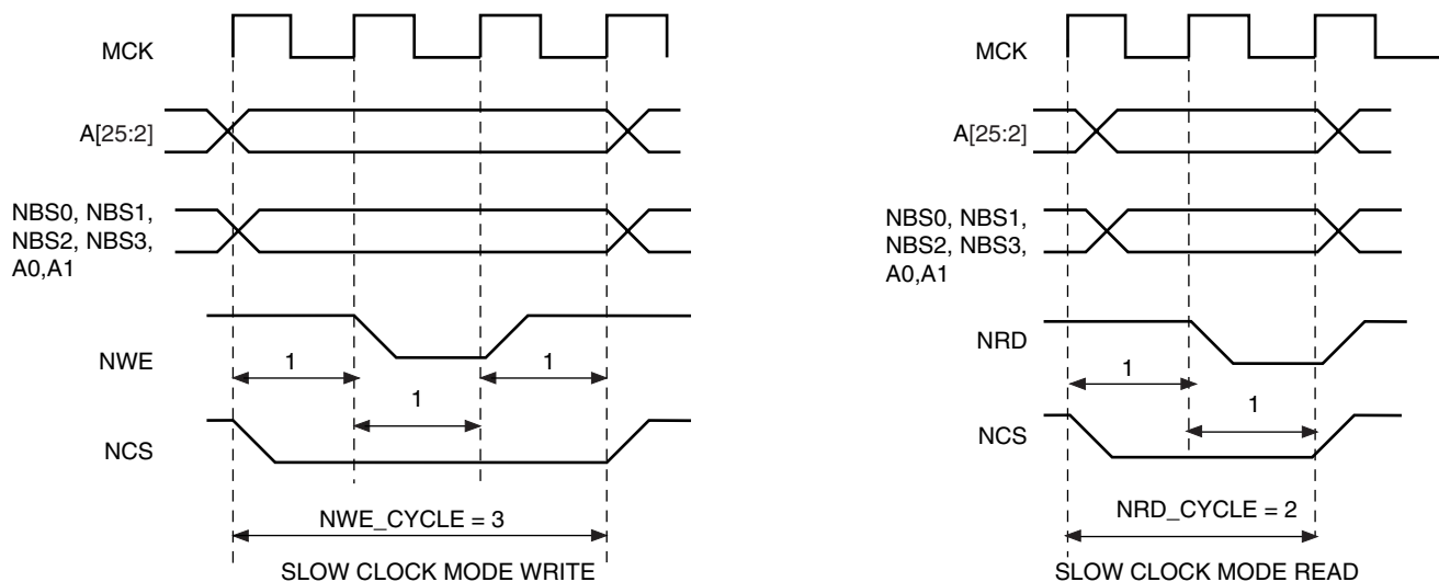
Figure 27-32. Read/write Cycles in Slow Clock Mode
