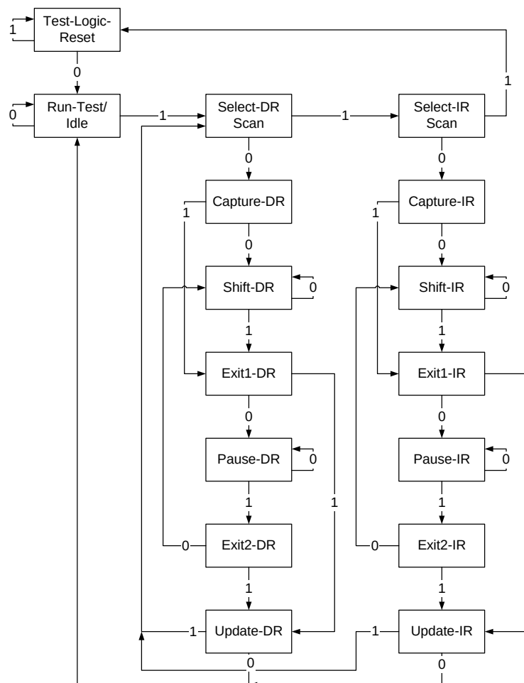
Figure 38-2. TAP Controller State Diagram
