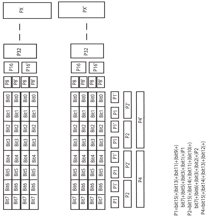
Figure 29-3. Parity Generation for 512/1024/2048/4096 16-bit Words
