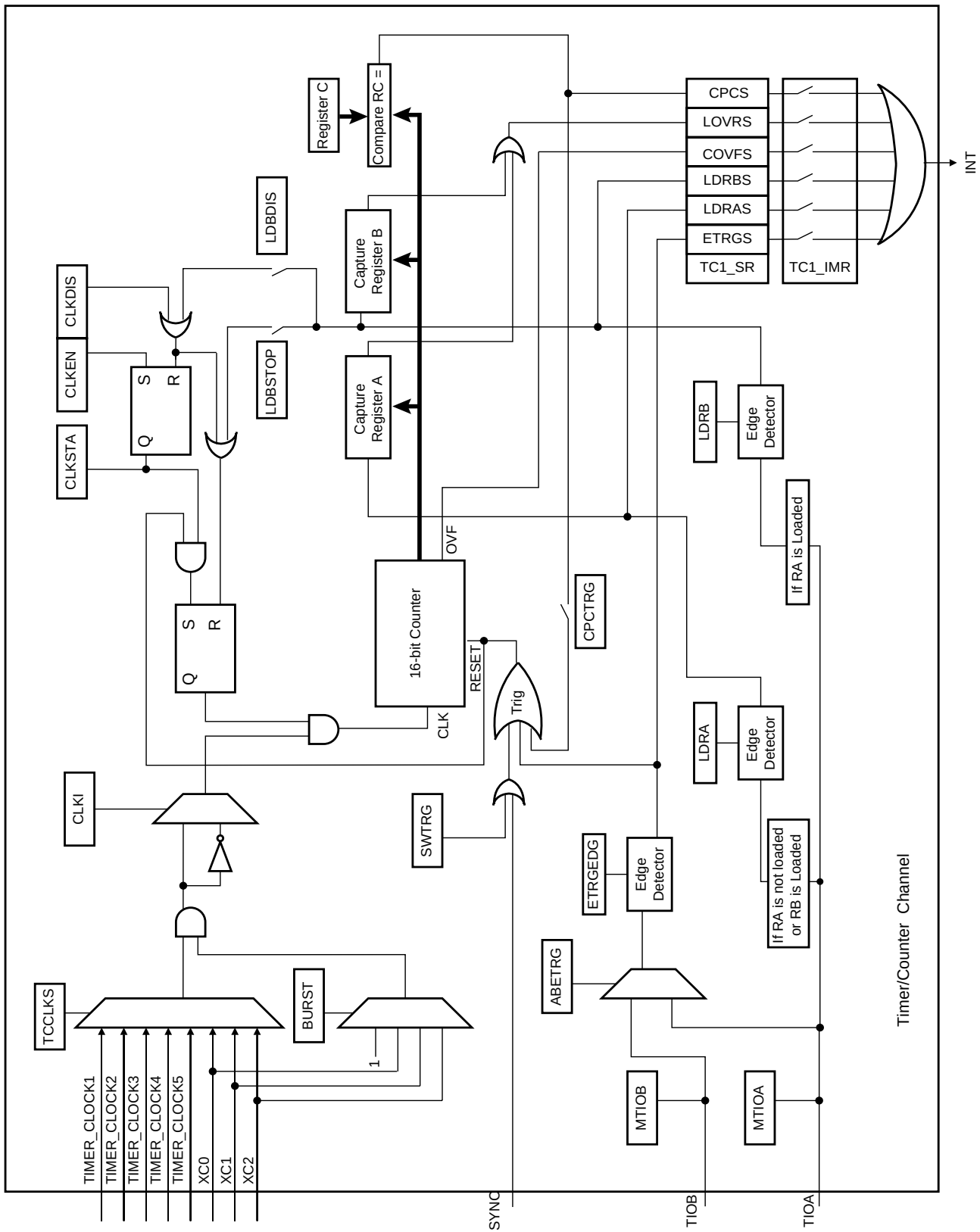
Figure 33-4. Capture Mode
