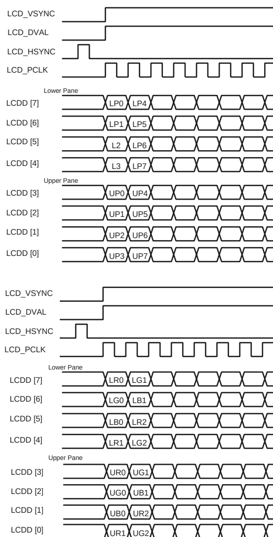
Figure 35-11. Dual Scan Monochrome and Color 8-bit Panel Timing (First Line Expanded View)
