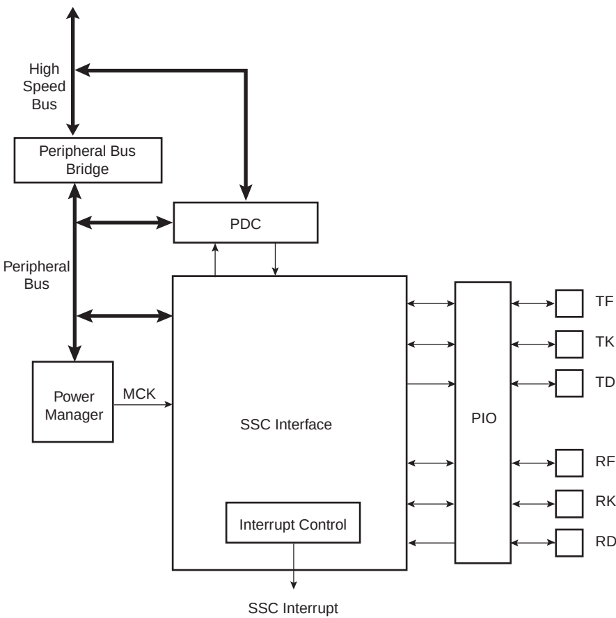
Figure 23-1. Block Diagram
