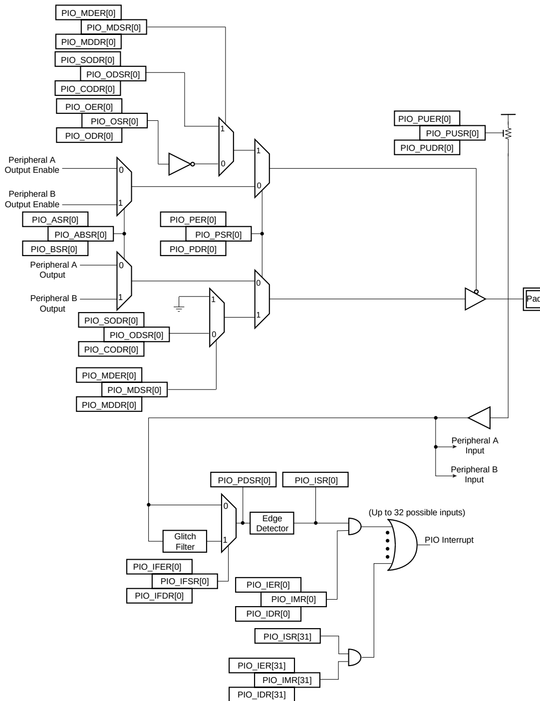
Figure 19-3. I/O Line Control Logic
