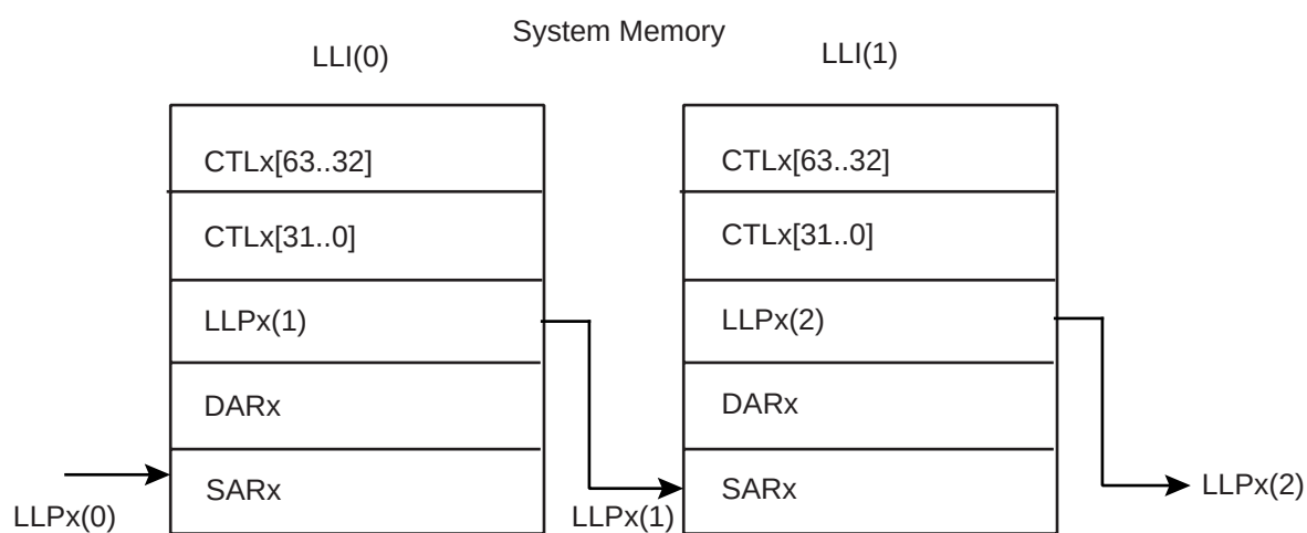
Figure 17-5. Multi-block Transfer Using Linked Lists
