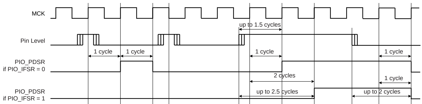
Figure 19-5. Input Glitch Filter Timing
