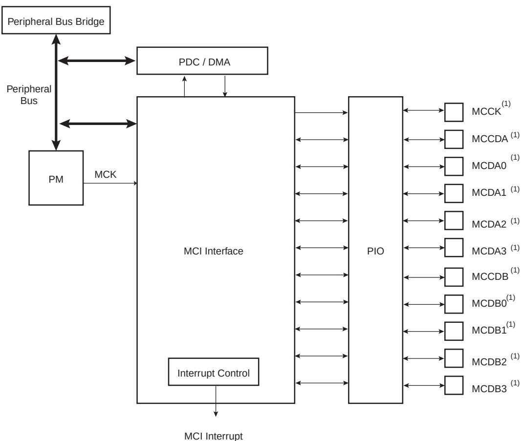
Figure 30-1. Block Diagram
